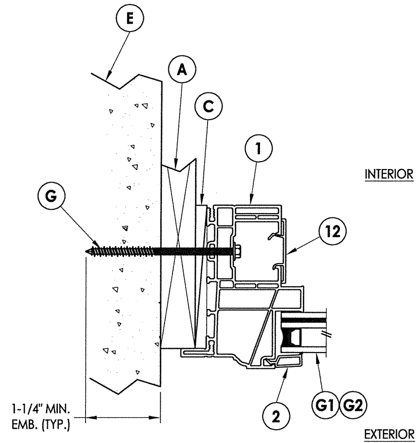
2 HORIZONTAL CROSS SECTION 2 1X Stud Construction
